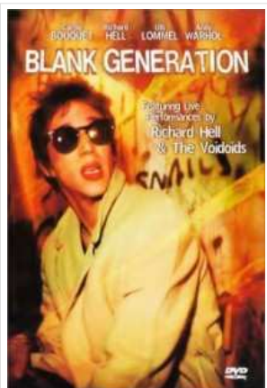
Blank Generation
